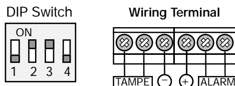
DIP Switch Configuration
